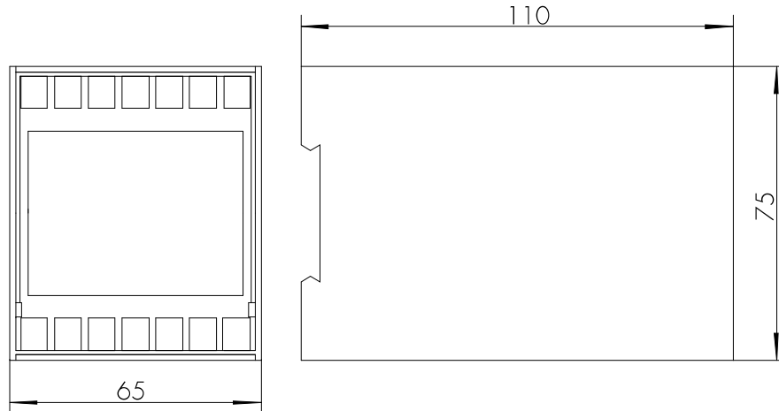
Figure 5.1: Dimensional drawings
